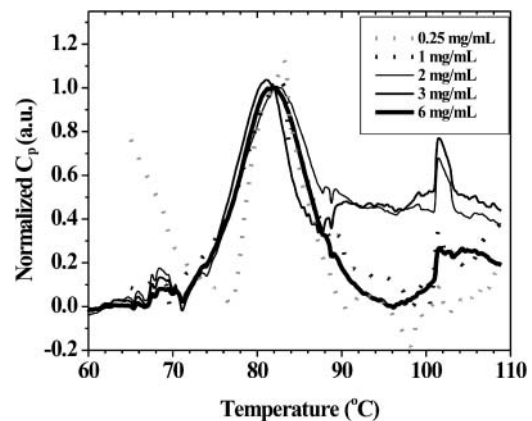
FIGURE 5 DSC of SA as a function of concentration. Data were obtained at 1°C/min for samples between 0.25- and 6-mg/mL concentrations.
