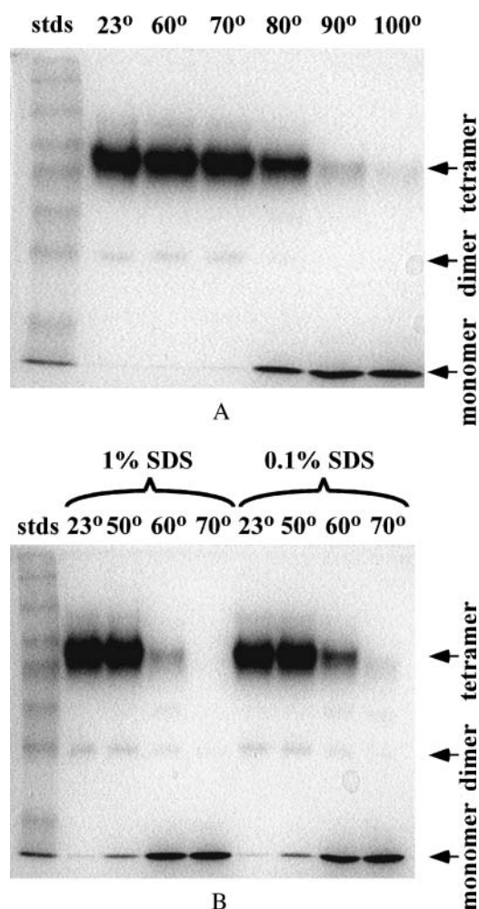
FIGURE 1 SDS-PAGE gels examining the effect of temperature and SDS on apparent oligomerization state of SA. (A) SA treated 3 min at indicated temperatures (°C). (B) Lanes 1–4, SA in 1% SDS; lanes 5–8, SA with 0.1% SDS at indicated temperatures (°C), respectively.
